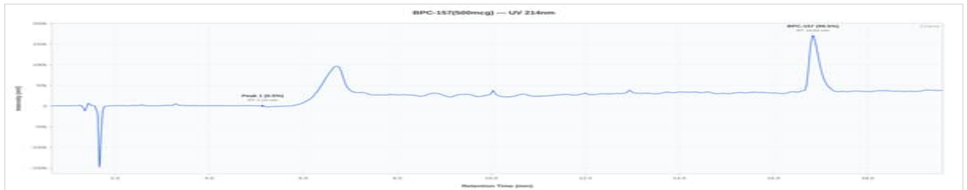
BPC-157 500mcg - 003-10-202601-001: UV Chromatogram
