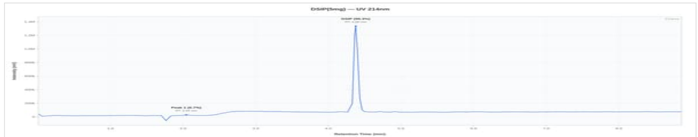
DSIP 5mg - 003-10-202601-001: UV Chromatogram
